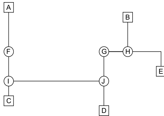
Figure 8.11 Minimal Length Steiner Tree
