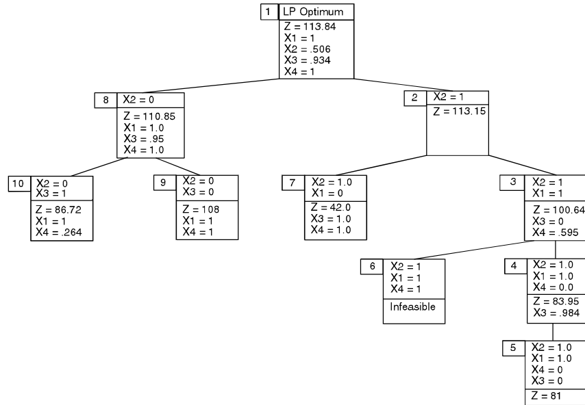
Figure 11.4 Branch-and-Bound Search Tree
